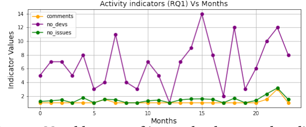
Figure 1: Monthly count of issues, developers and median comments which mention PRs and fixes for Maven.
